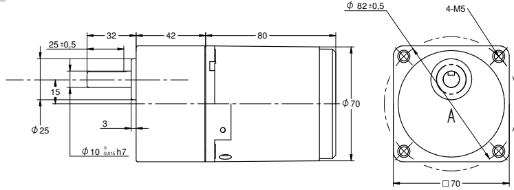
DRAWING (mm)
